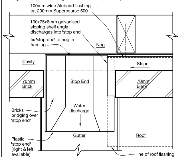
FIG.5 BASE OF SLOPING SHELF ANGLE - Plan View Large Stop End (eg Gerrard Stop End)
