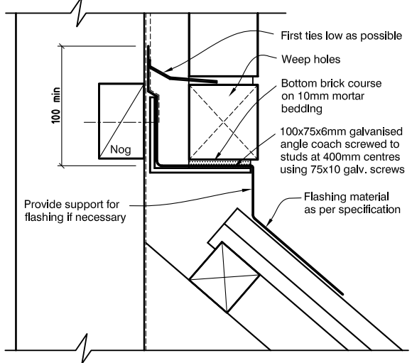
FIG.8 TOP OF ROOF SLOPE
