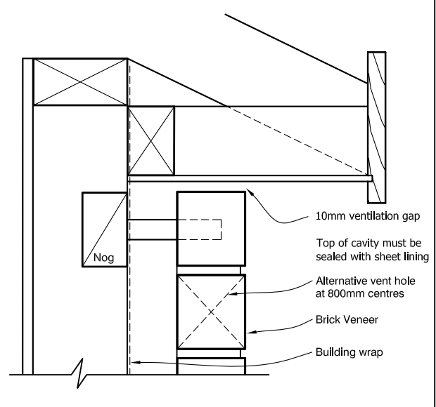
FIG.18 FLAT SOFFIT
